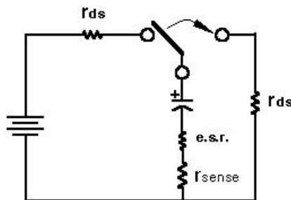
Fig. 3 Capacitor Transient Response Measurement Circuit
